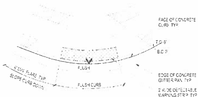
Sidewalk Access Ramp
